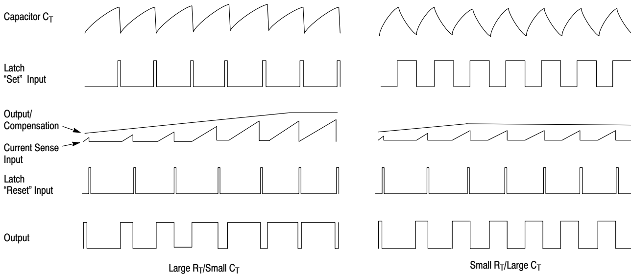
Figure 19. Timing Diagram
